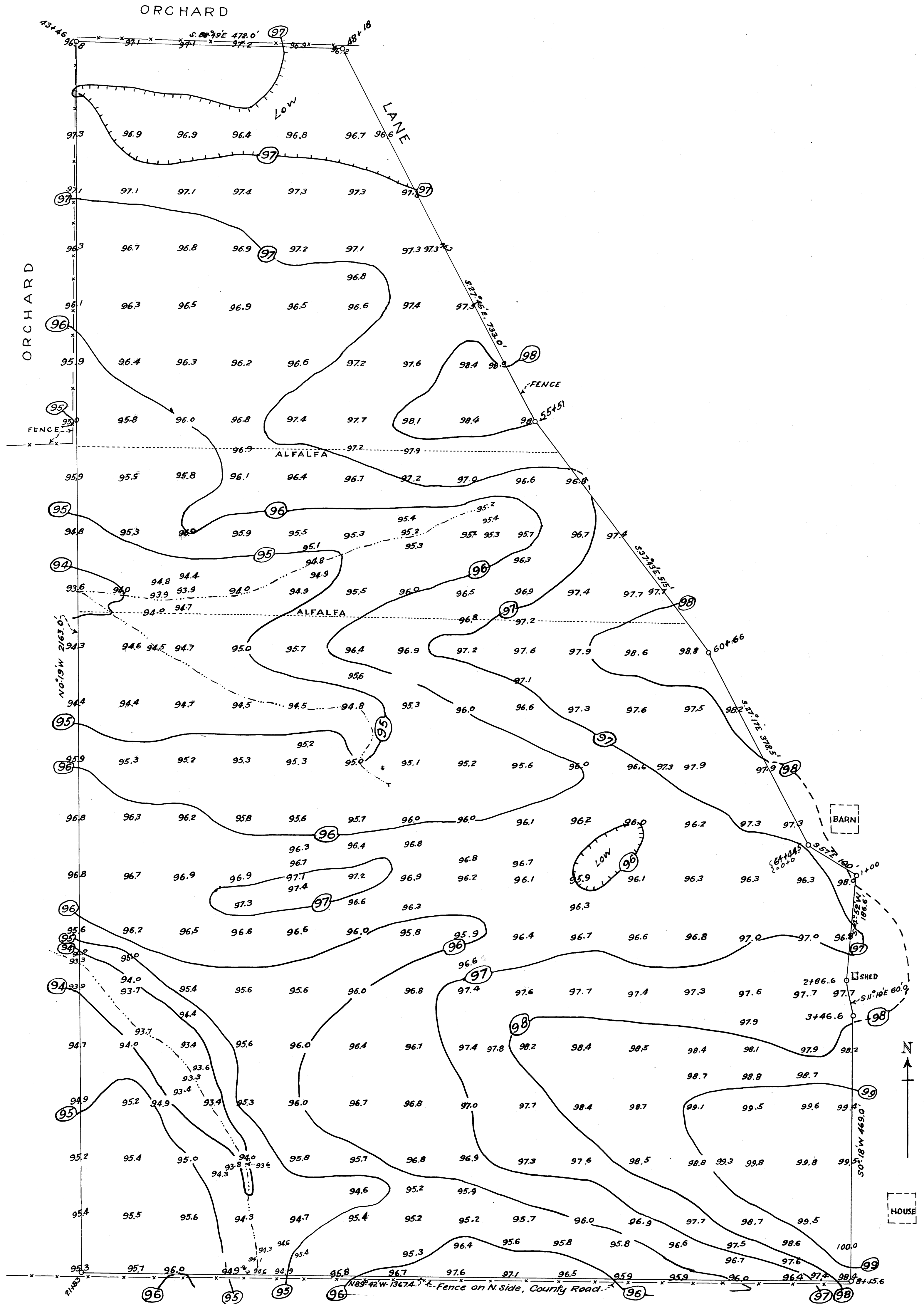
CONTOUR MAP, 51.96 Ac; SHAMBROOK RCH. IN E 2 Sec. 25, T. 25 S., R. 7 W., - Map Co. Road No. 6.
