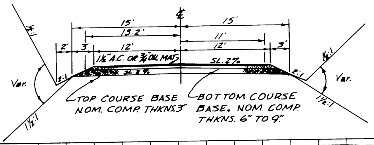
TYPICAL SECTION
