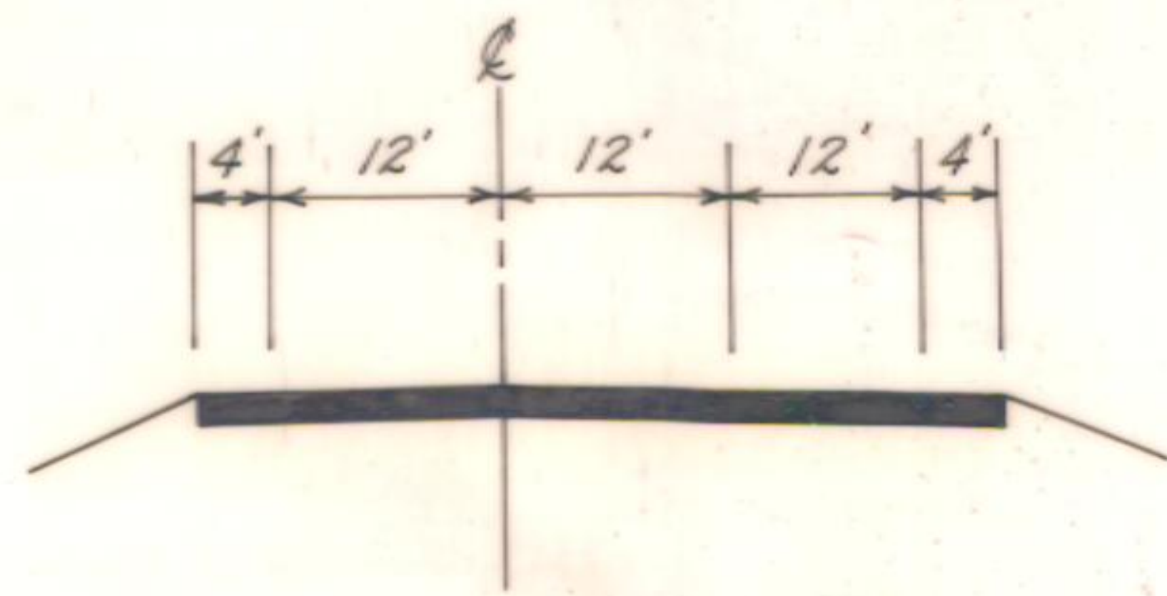
TYPICAL SECTION LEFT OR RIGHT
