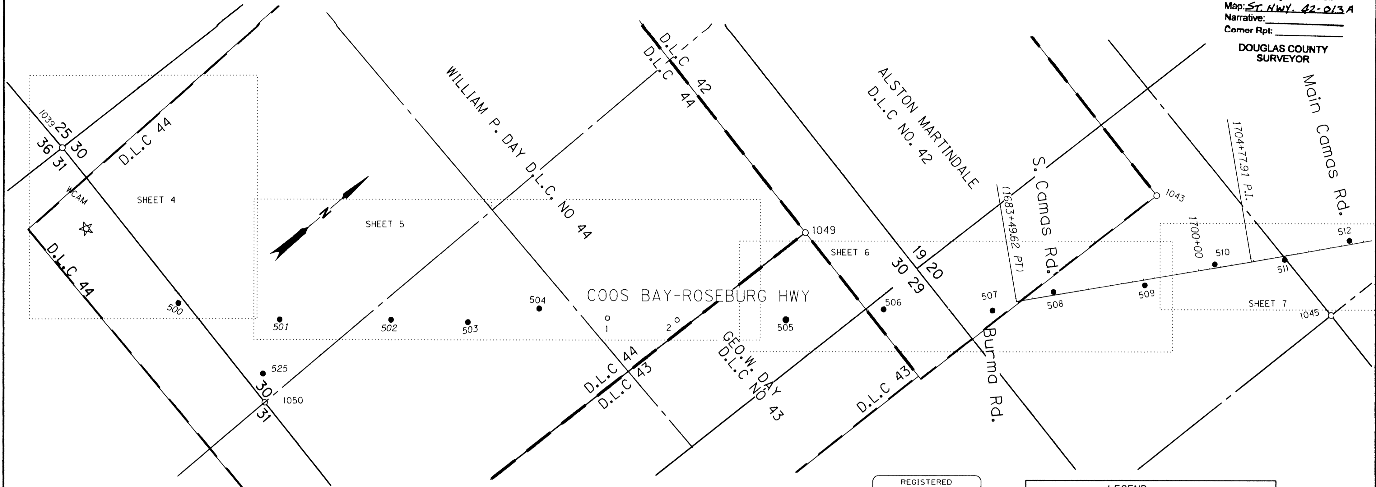
CONTROL NETWORK SCHEMATIC NOT TO SCALE
