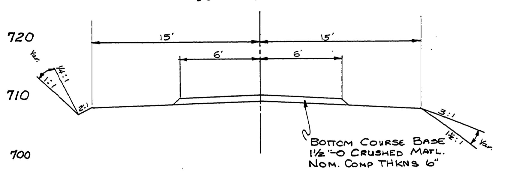
Typical Section
