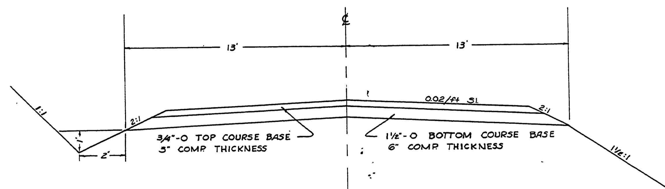
TYPICAL SECTION
