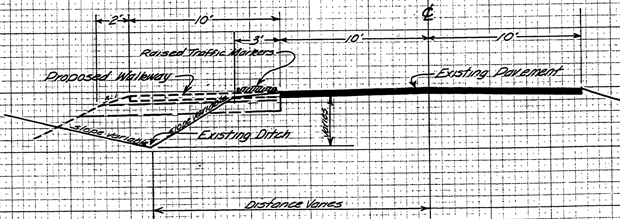
TYPICAL SECTION STA. 0+00 to 17+25 SCALE - 1" = 4'
