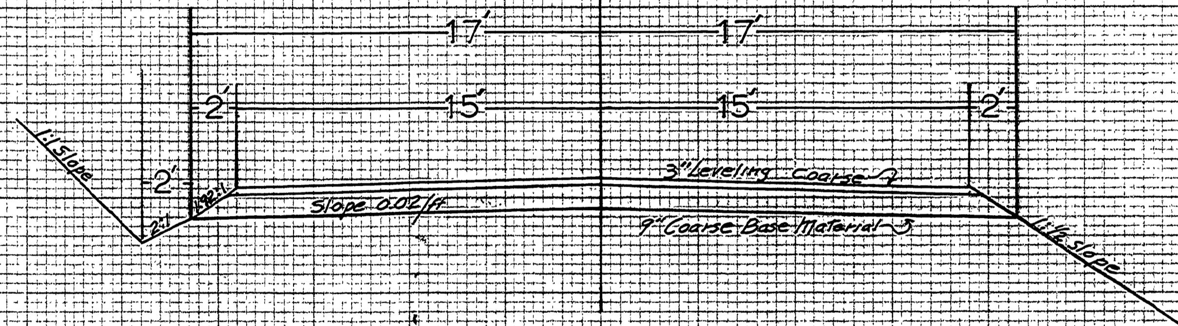
TYPICAL SECTION
