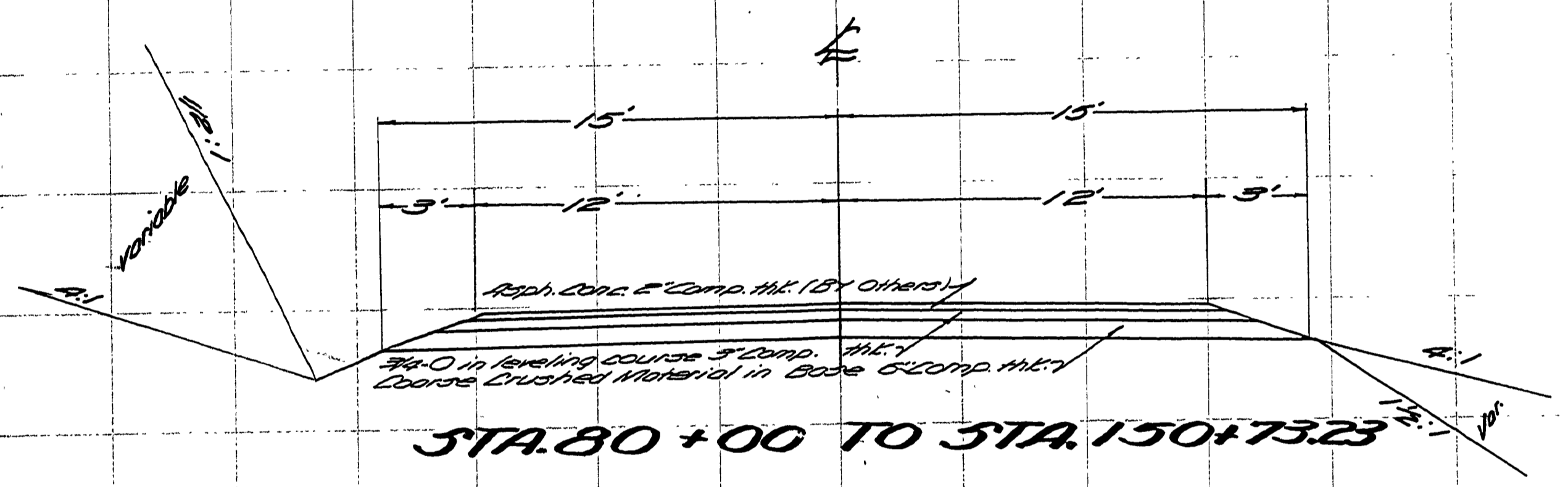
TYPICAL SECTION
