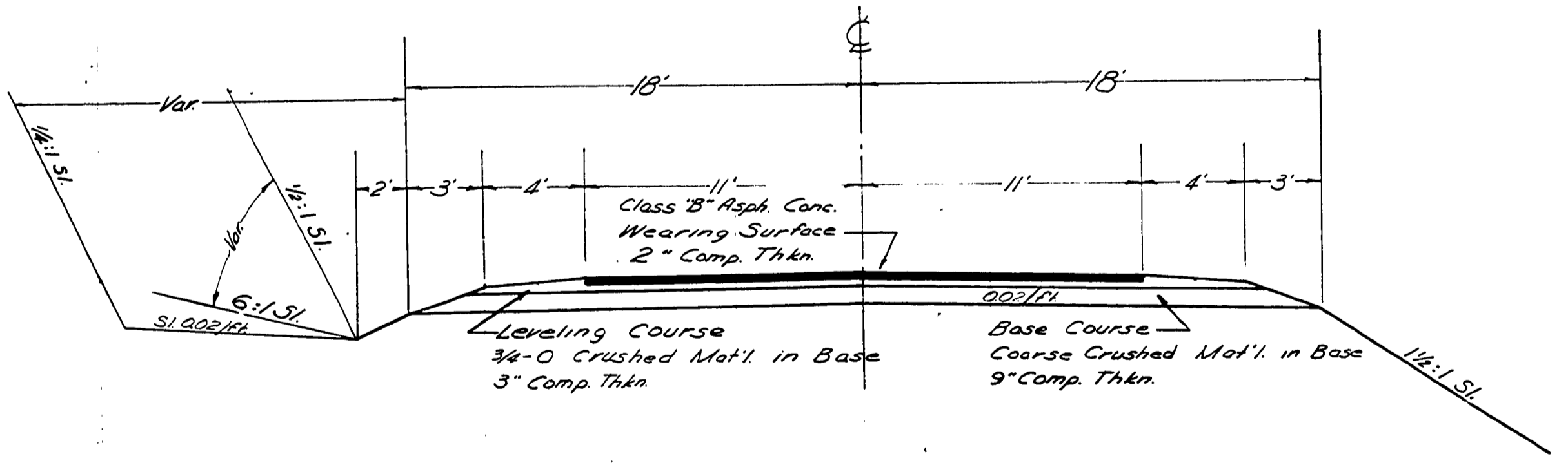
TYPICAL SECTION
