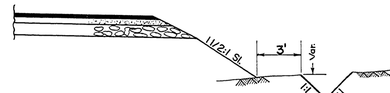
TYPICAL DITCH RT. STATION 307+00 TO STATION 316+50
