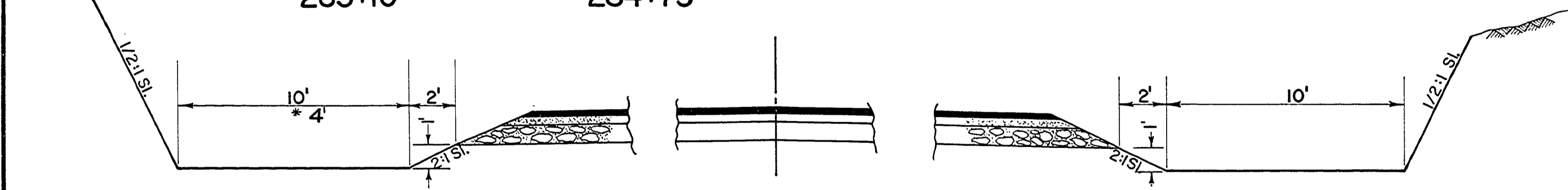
FALLOUT SECTION STATION 317+50 TO STATION 321+00 * STATION 305+50 TO STATION 308+50
