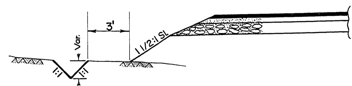
TYPICAL DITCH LT. STATION 189+00 TO STATION 190+50 283+10 284+75
