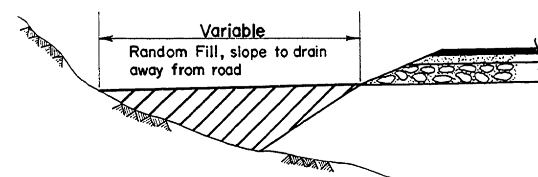
RANDOM FILL AREA LT. STATION 311+50 TO STATION 316+00 ± 297+00 TO 300+50 ±
