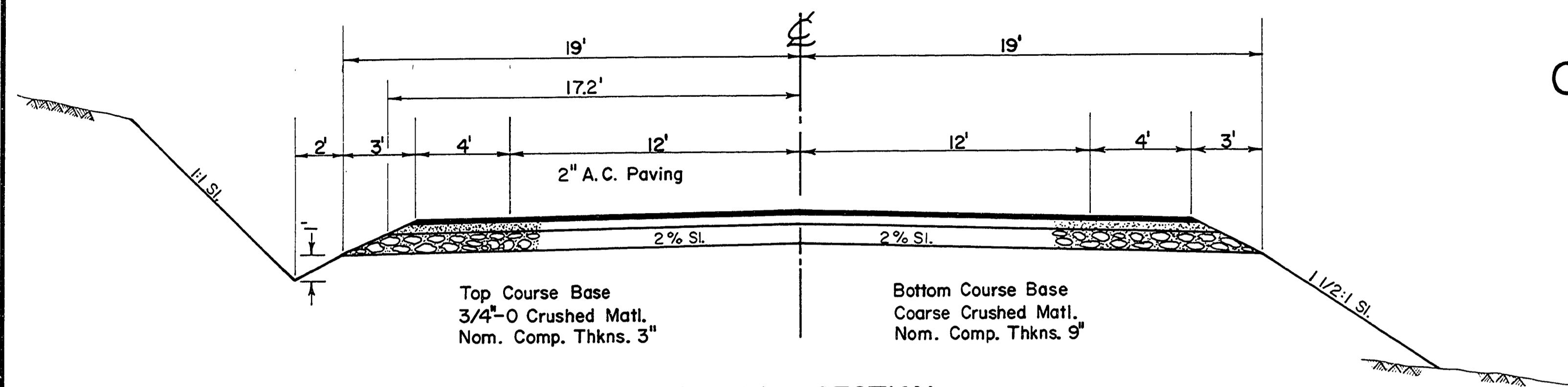
TYPICAL SECTION STATION 176+50 TO STATION 324+00
