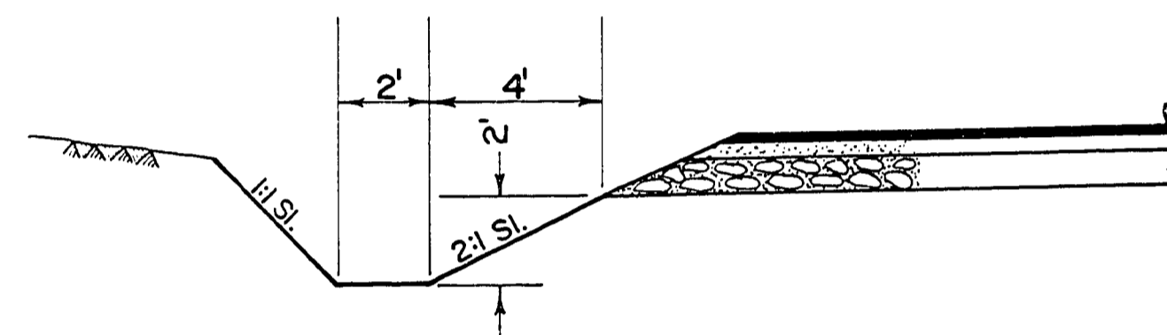
TYPICAL DITCH LT. STATION 253+50 TO STATION 264+00
