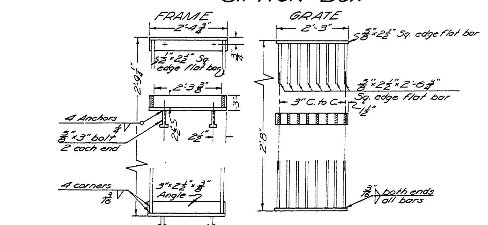
DETAILS FOR FRAME & GRATE OF SIPHON BOX
