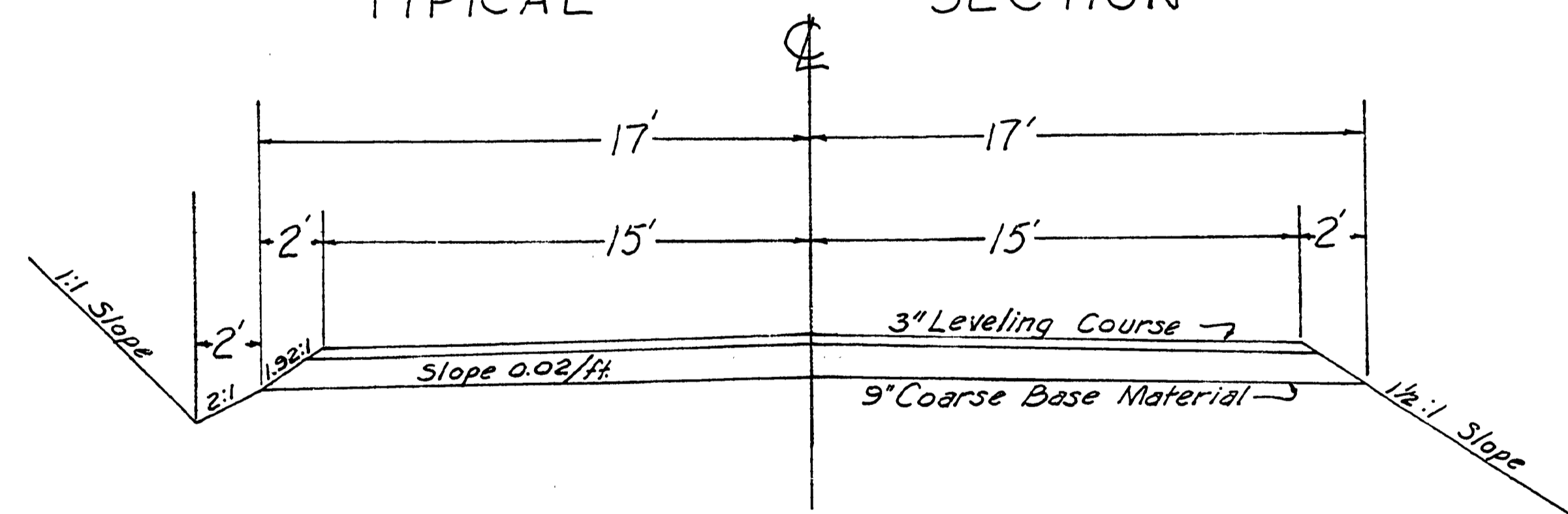
TYPICAL SECTION
