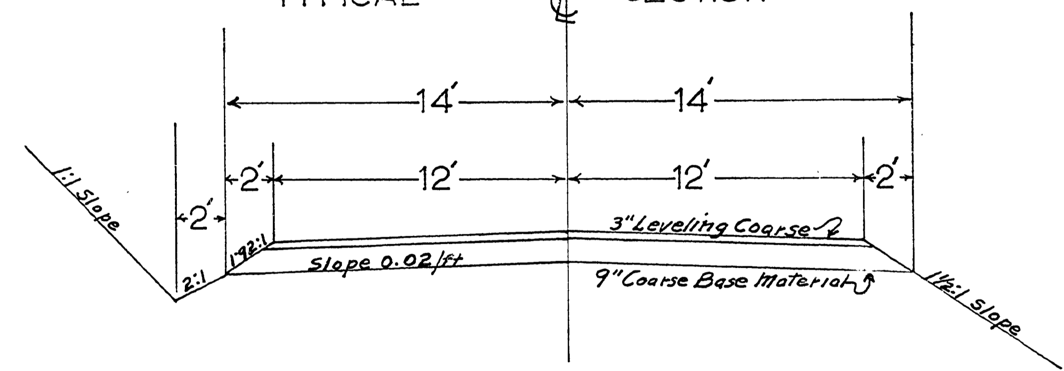
TYPICAL SECTION
