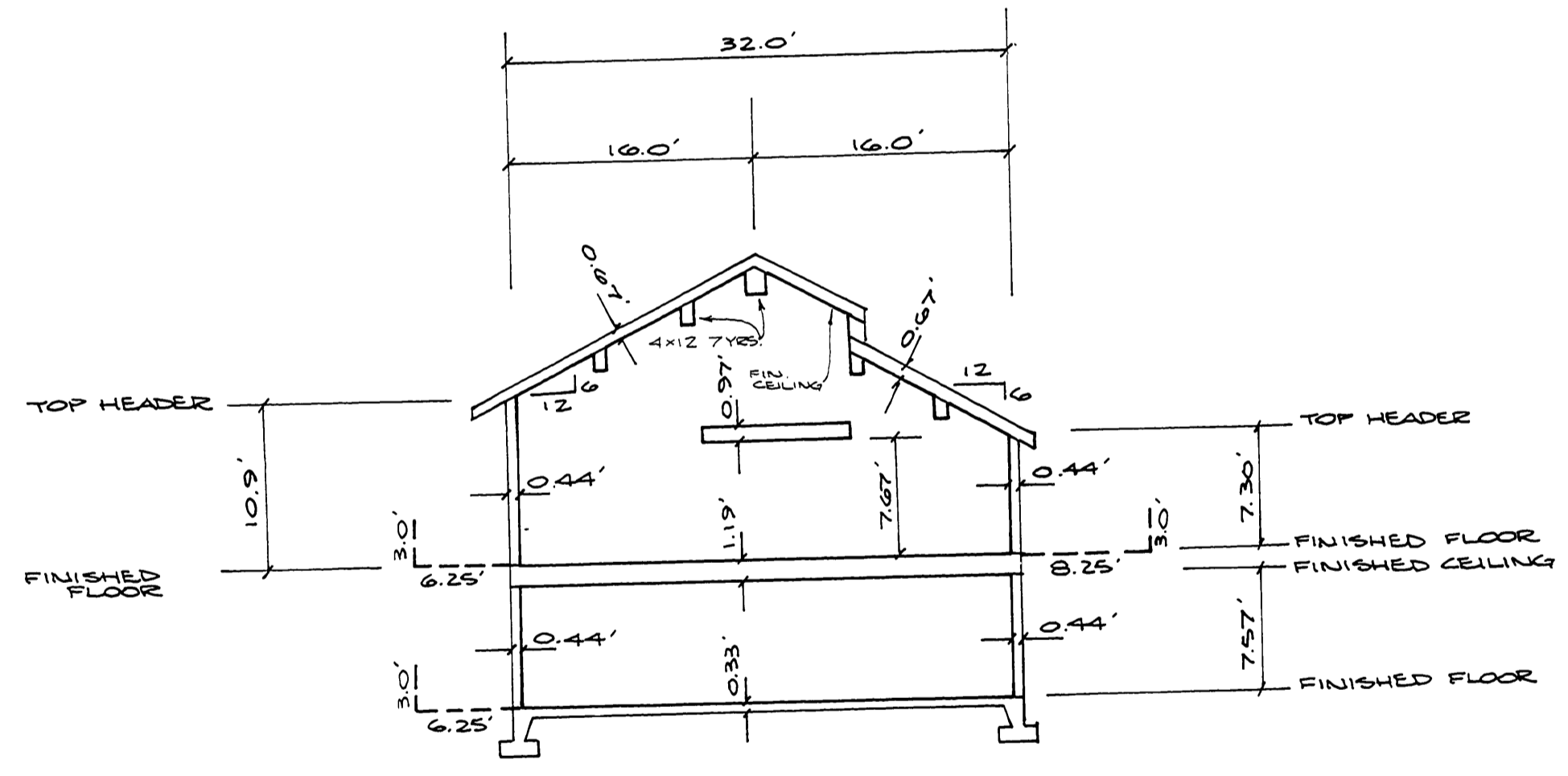
TYPICAL SIDE VIEW SCALE: 1" = 10'
