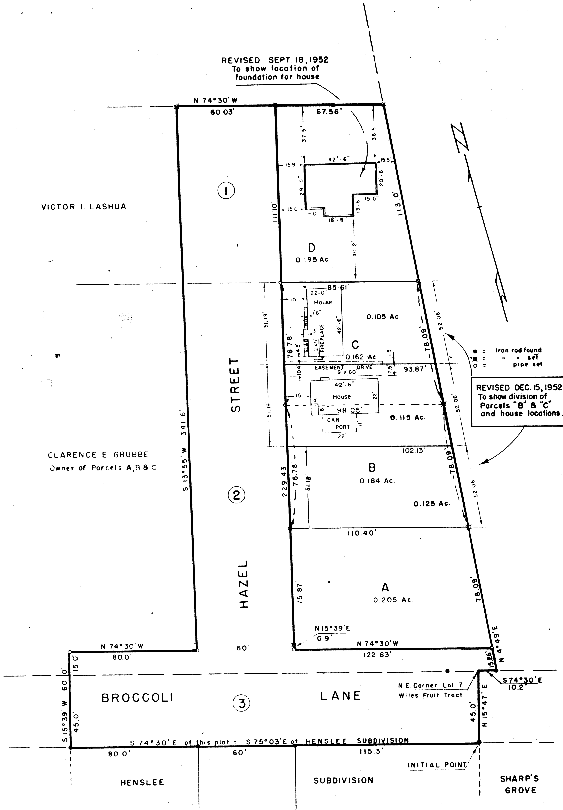
A PLAT OF CERTAIN PARCELS within Lot 6, Wiles Fruit Tract, T 27 S - R 6 W W.M. Douglas Co. Ore. March 1952 Scale 1" = 30
