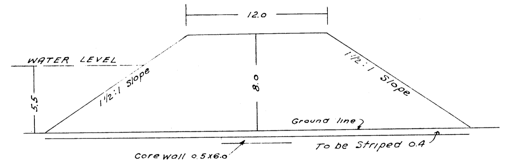
TYPICAL DYKE SECTION
